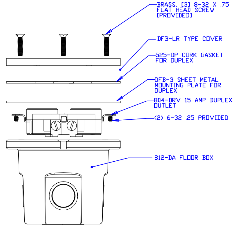
RIGHT [EXPLODED]
