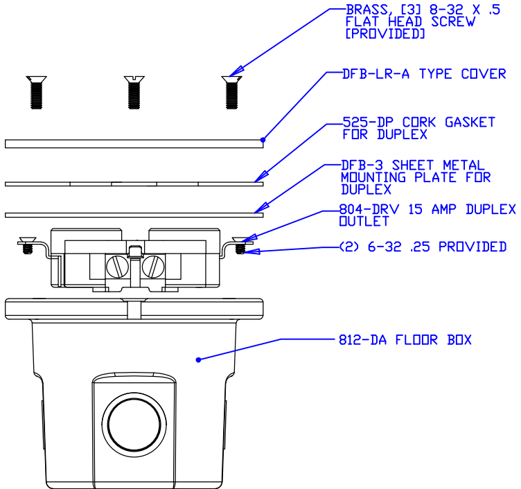
RIGHT [EXPLODED]
