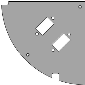
DB15x2 Connector Plate
