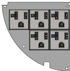
Power 5 Connector Plate (15A or 20A Single Receptacles)
