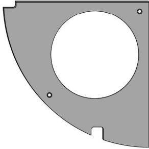
2" NPS Connector Plate
