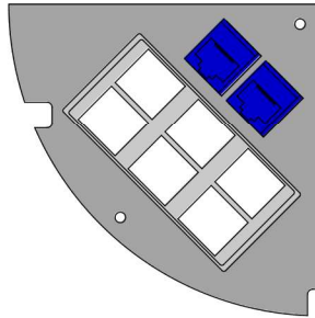
DPC-Comm 2 Connector Plate
