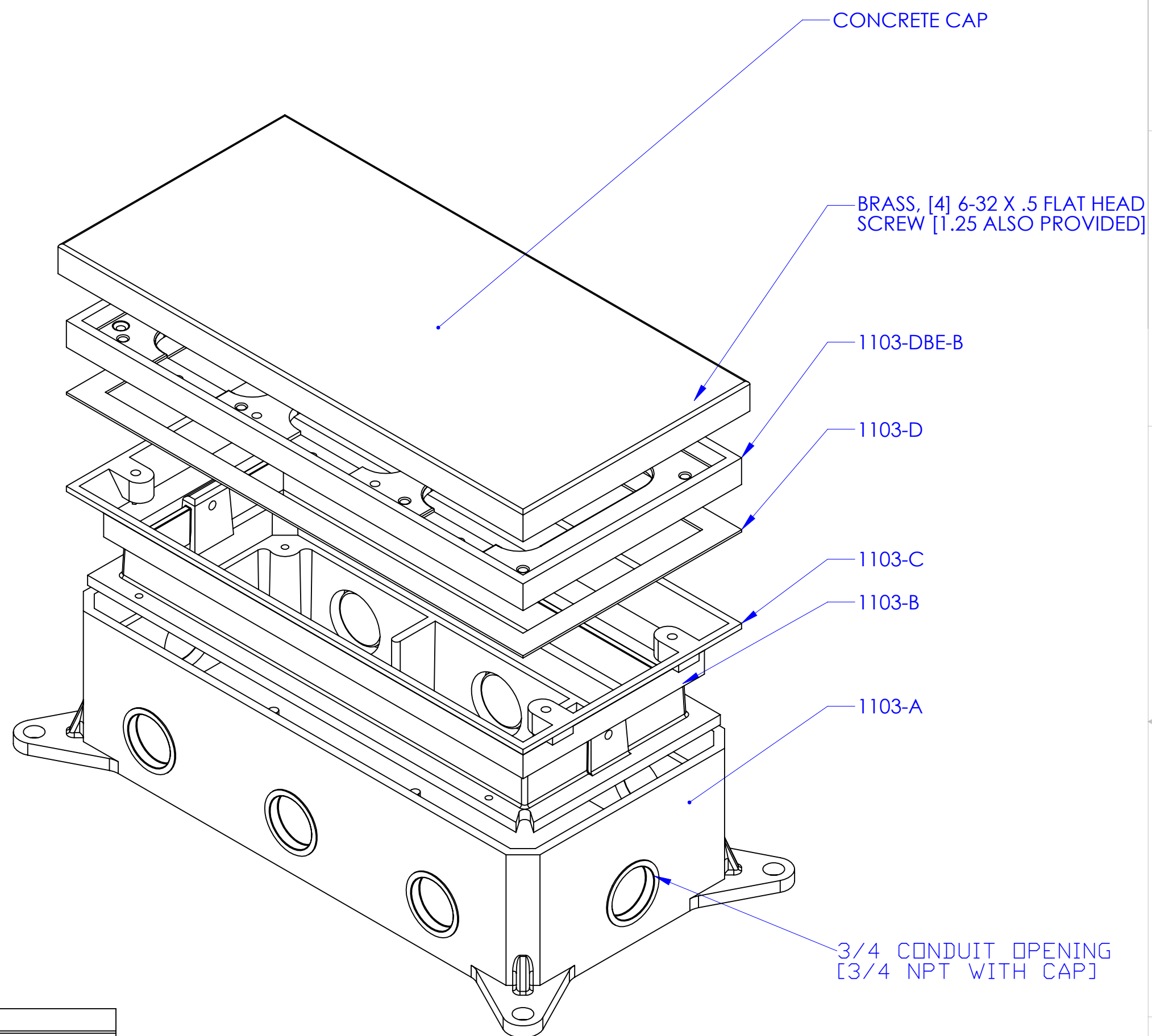
EXPLODED VIEW
